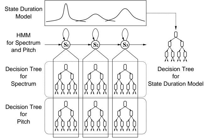
Figure 2. Decision trees.
